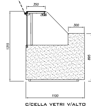
C/CELLA VETRI V/ALTO
