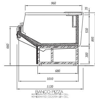
REFRIGERATO CON CELLA REFRIGERATED COUNTER WITH CELL REFRIGERATED COUNTER WITH CELL
