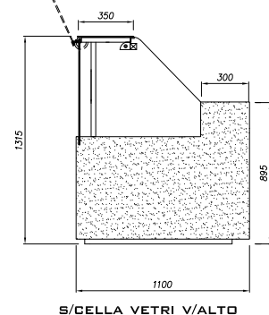
S/CELLA VETRI V/ALTO
